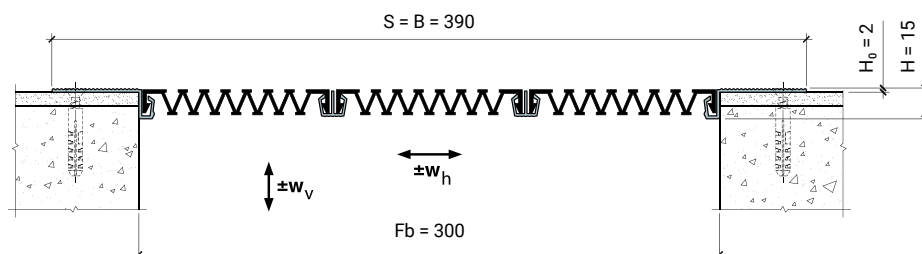
MANGRA 3210-300
